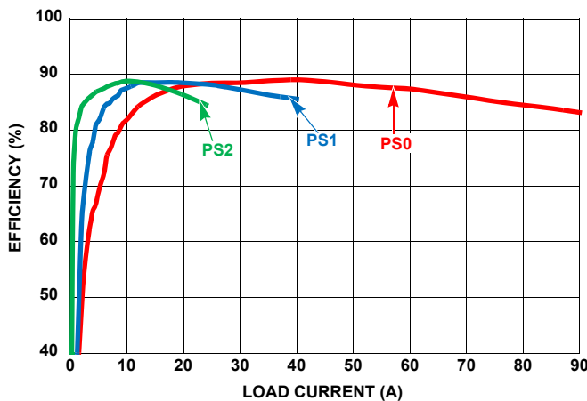
FIGURE 1. VR A EFFICIENCY vs LOAD
